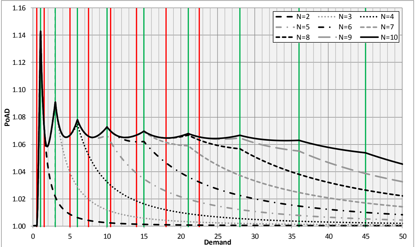
Figure 2: PoAD vs Demand for N -Parallel Link networks and UE (Green) and SO (Red) Link Activation Points
